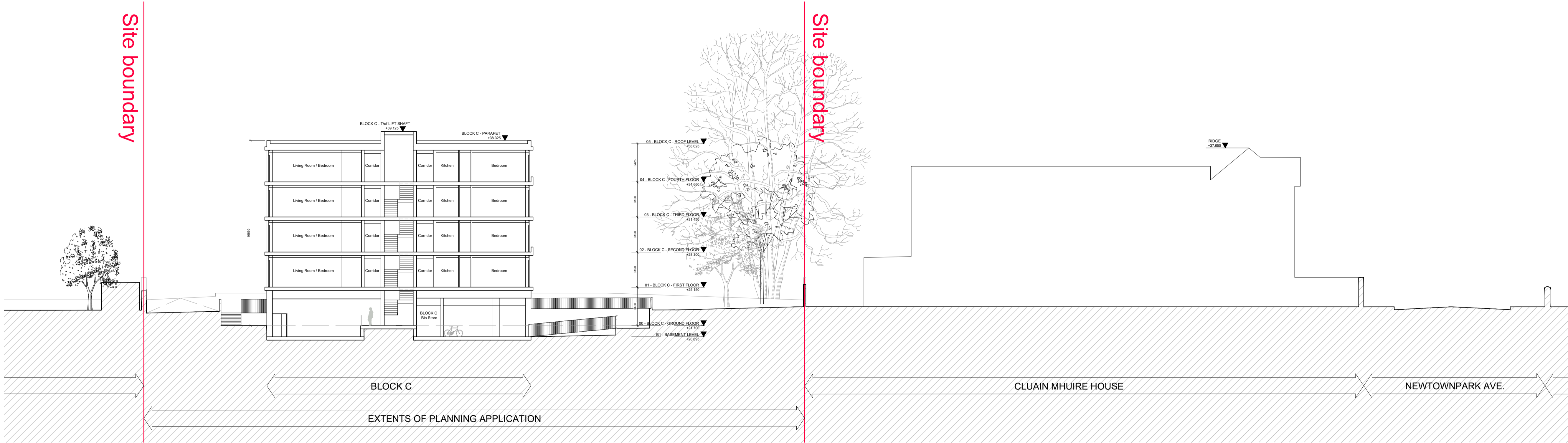
Section DD Block C - PROPOSED
