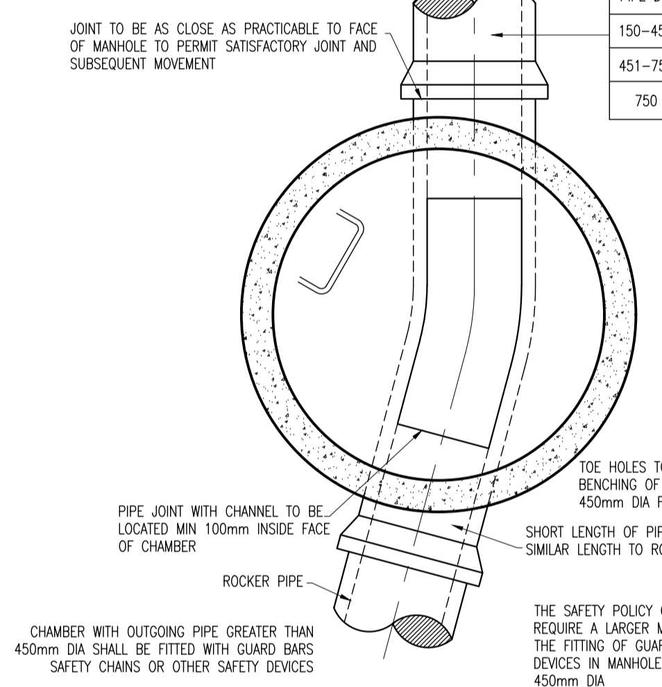
TYPICAL MANHOLE DETAIL - TYPE J DEPTH TO SOFFIT 1.35 TO 3m SCALE 1:25
